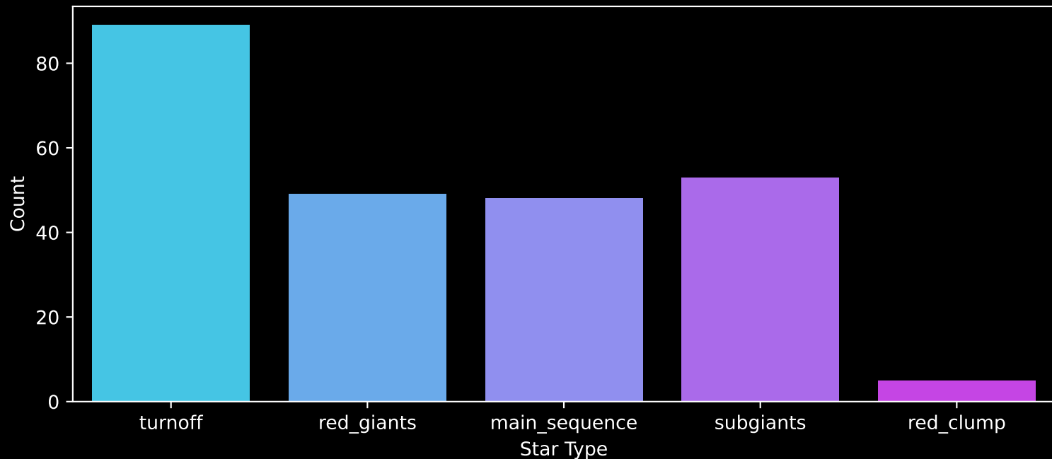
GALAH DR4 Field: [9221] Count plot of Star Type
