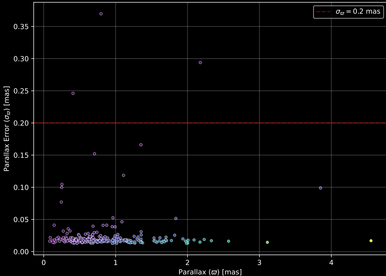
GALAH DR4 Field: [9221] Parallax Quality (n= 244)
